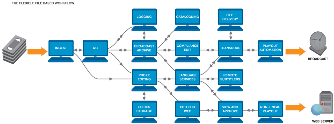
Fig 3. The flexible file based workflow.
